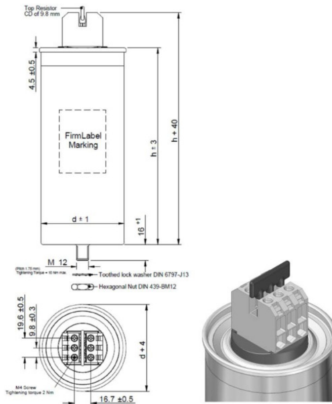
Terminal type B: Capacitors with Sigut terminal
